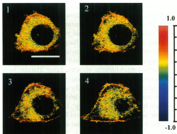
FIGURE 6 Four GP cross sections of a single mouse fibroblast cell labeled with Laurdan. The distance between subsequent frames is 1\ \mu\text{m} . A 100 \times 1.25 N.A. oil immersion Zeiss objective was used. The laser pixel dwell time is \sim 300\ \mu\text{s} . Features of GP domains can be seen. The scale bar is 10\ \mu\text{m} .
